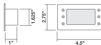
LED Light Engine
