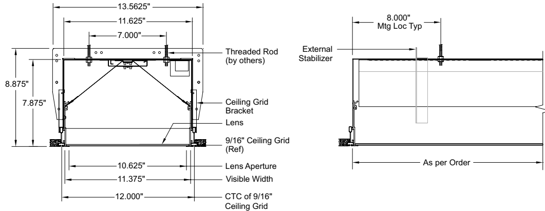
Ceiling Trim Detail
